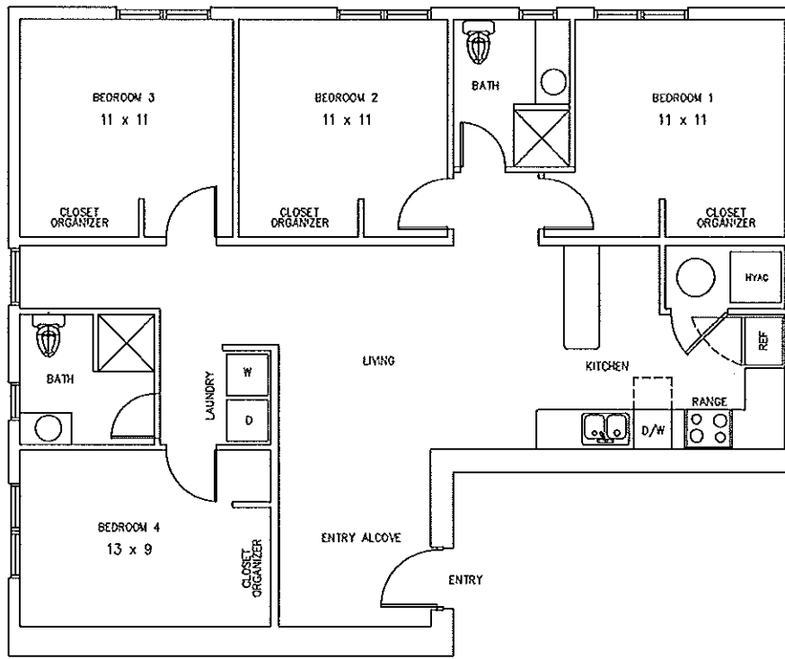
SECOND FLOOR
